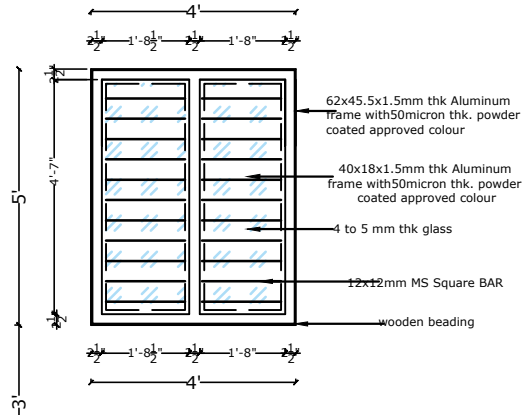
W(4'-0"x5'-0") SILL LVL. 3'-0"
