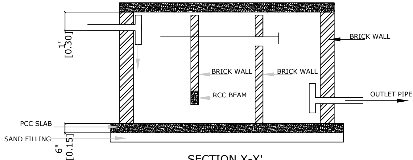
SECTION X-X'
