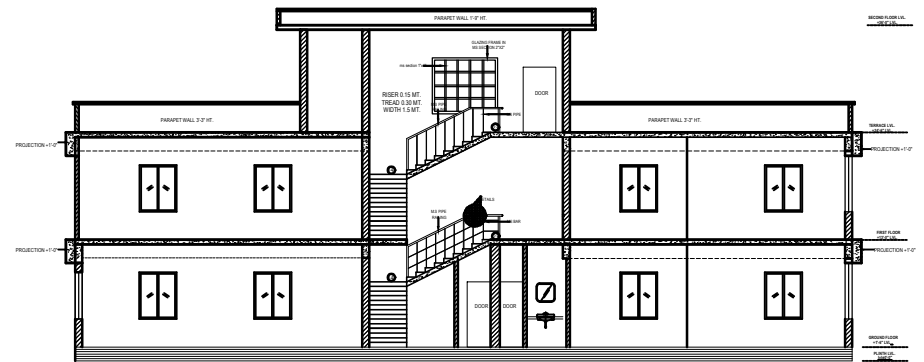
SECTION ELEVATION AA'
