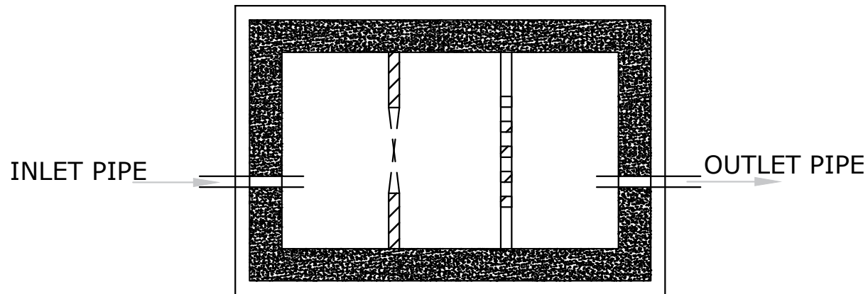
SEPTIC TANK 3.3M X 2.1M X1.8 M
