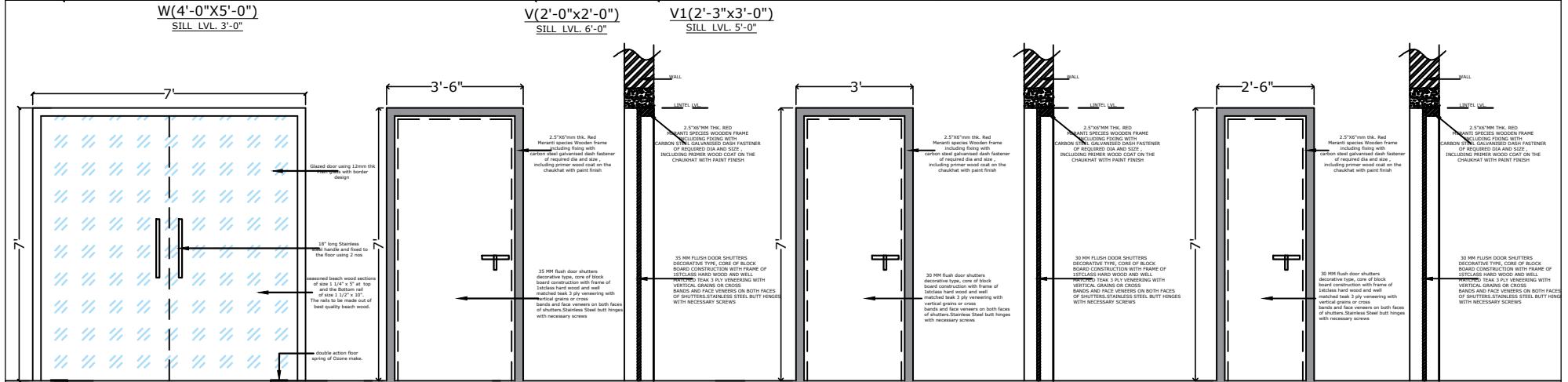
GROUND FLOOR DOOR WINDOW DETAIL
